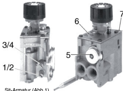
Sit-Armatur (Abb. 1)
